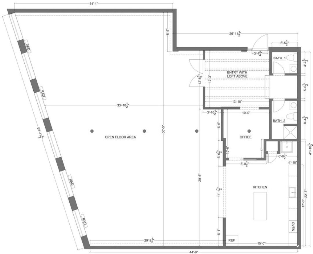
A EXISTING PLAN 1/4" = 10"
